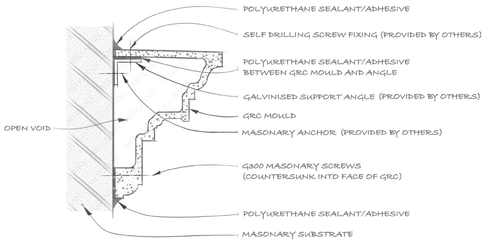
G.R.C. MOULD FIXING DETAIL (SUPPORT ANGLE)
