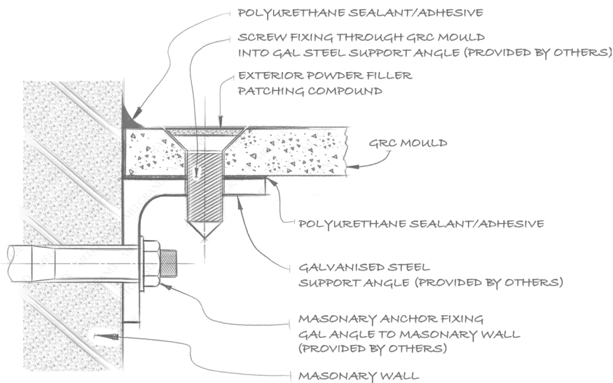
SUPPORT ANGLE FIXING DETAIL FOR HOLLOW G.R.C. PARAPET MOULD
