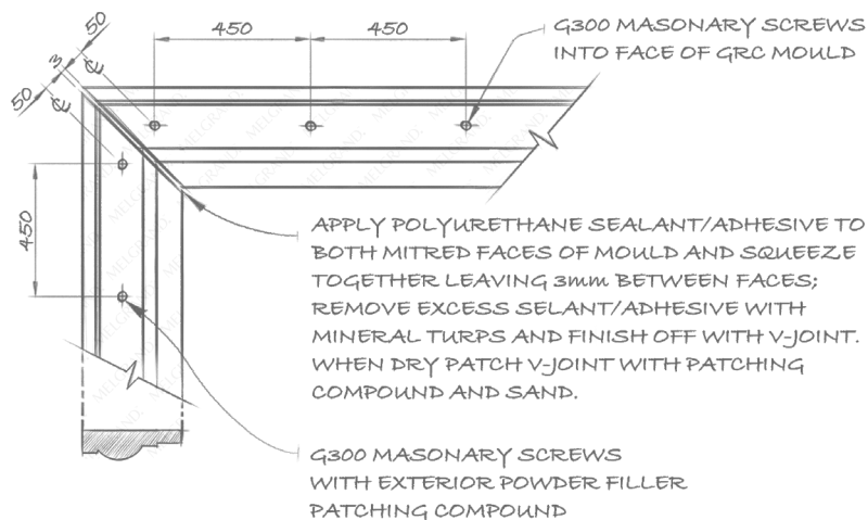
FIXING DETAIL FOR SOLID GRC MOULD
