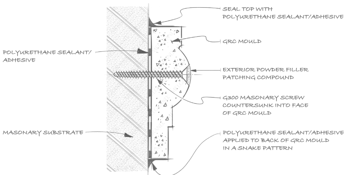
FIXING DETAIL FOR SOLID GRC MOULD
