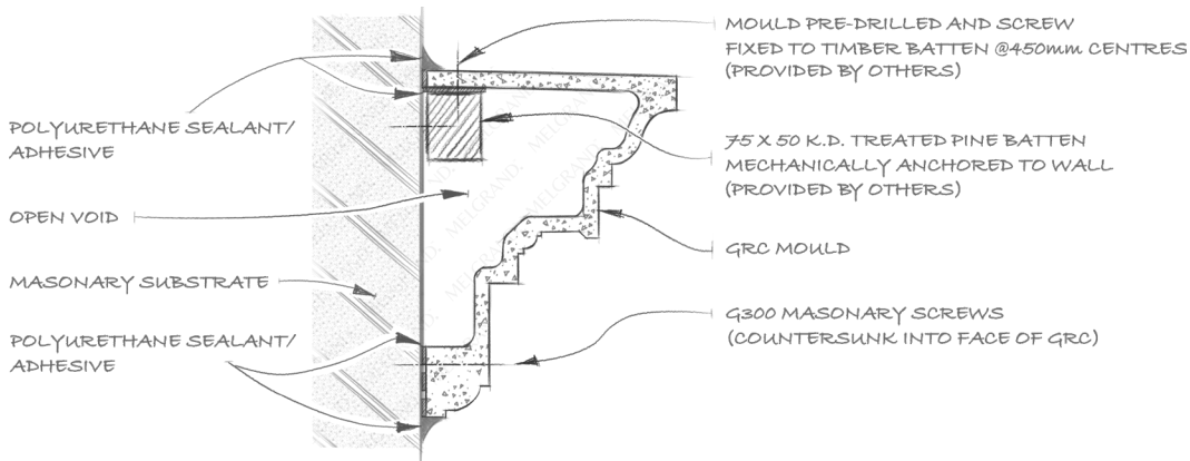
G.R.C. MOULD FIXING DETAIL (TIMBER BATTEN)
