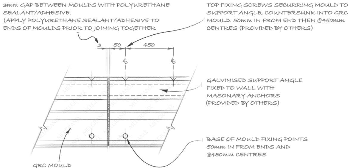
FIXING DETAIL FOR HOLLOW GRC PARAPET MOULD
